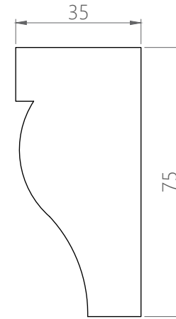
HORN H-6
