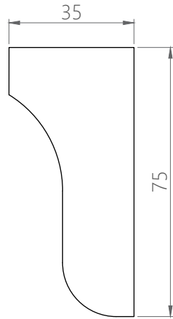
HORN H-3
