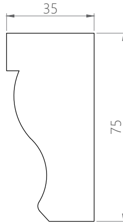
HORN H-4
